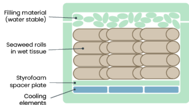
Schematic of Sori shipment box build-up
